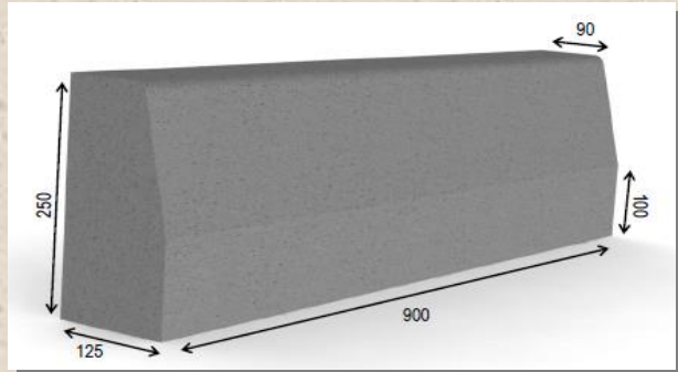
Standard Road Kerb
